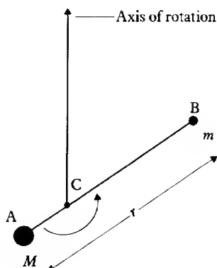
1.17 Bohr model with finite nuclear mass.
